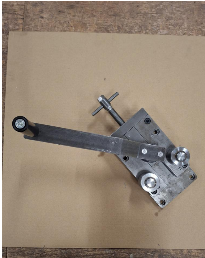
Rollbieger / Roll Bender – made by berufl. Schulen Altötting/Vocational School Altötting
